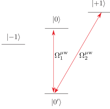
FIG. 2: Two bases of quantum states are used. The coupled basis comprises |0'\rangle and the magnetic field sensitive state |+1\rangle . The uncoupled basis encodes the qubits and is formed by magnetic field insensitive states |0\rangle and |0'\rangle , which belong to different hyperfine manifolds. An ion is brought to the uncoupled basis to suppress its interaction with the other ions.
